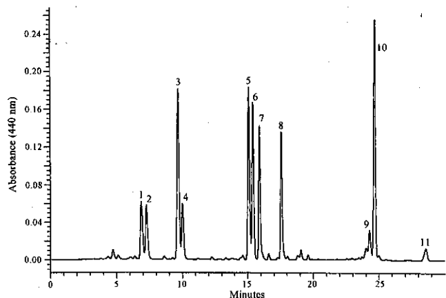
Figure 2 Chromatogram of a mixture of acetic extracts obtained from Emiliania huxleyi and Isochrysis galbana . Column: Symmetry C8, Eluents: (A) methanol: 1M ammonium acetate, 75:25 (v:v); (B) methanol. Gradient: linear from 0 to 100 % B in 20 min., then kept at 100 % B during 10 min. Temperature: 25 °C. Flow rate: 0.8 mL min -1 . Peak identification: 1 = DV-Chl c 3 ; 2 = MV-Chl c 3 ; 3 = Chl c 2 ; 4 = Chl c 1 ; 5 = fucoxanthin; 6 = 19'-hexanoyloxyfucoxanthin-like pigment; 7 = 19'-hexanoyloxyfucoxanthin; 8 = diadinoxanthin; 9 = apolar Chl c from Emiliania huxleyi ; 10 = MV-Chl a ; 11 = β,β-carotene.
